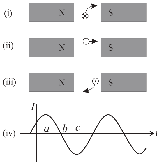
Fig. 12.8 (b): Wave form generation.
