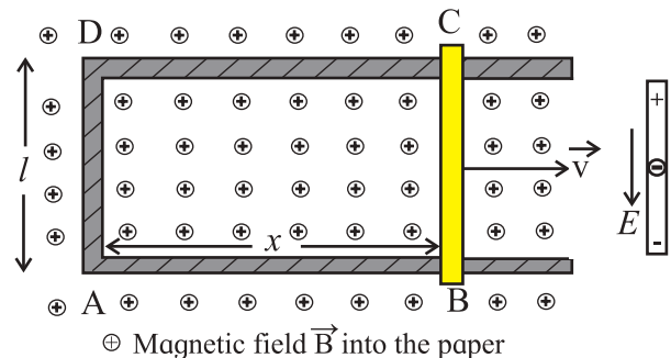
Fig. 12.5: A frame of wire ABCD in magnetic field \overrightarrow{B} . Wire BC is moving with velocity \vec{v} along x- axis.
