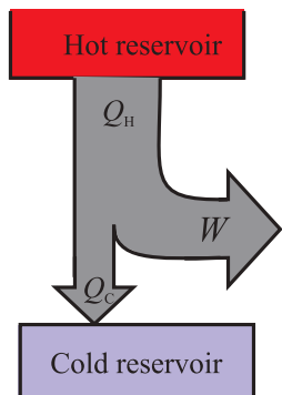
Fig. 4.25 (a): Second law of thermodynamics.
