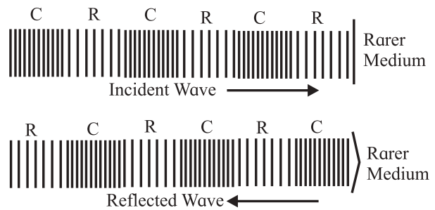
Fig. 6.5: Reflection of a longitudinal wave from a rarer medium.
