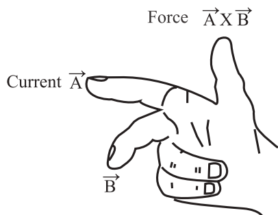
Fig. 10.11: The right hand rule.
