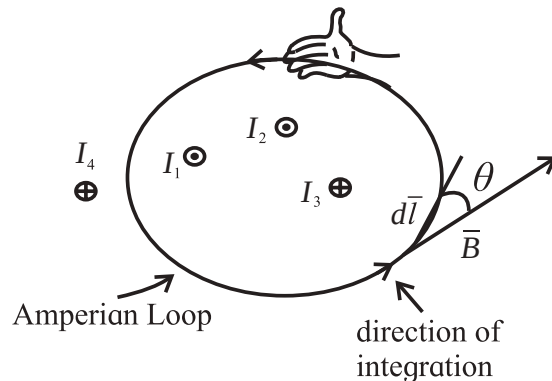
Fig. 10.22: Amperian Loop.
