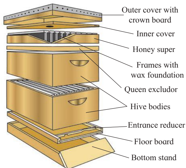
Fig. 11.6 : Artificial bee hive
