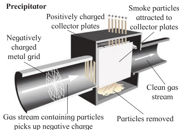
Fig. 15.4 : Electrostatic precipitator
